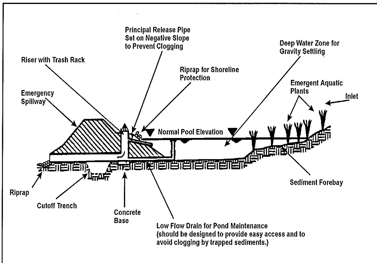
FIGURE 1 TYPICAL LAYOUT OF A WET DETENTION POND
